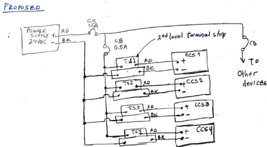
Fig.2. Proposed wiring connection to power Constant Current Source boards
